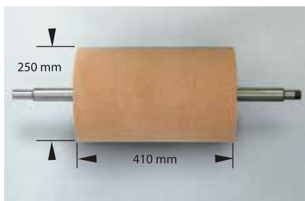
Assembled grinding stone with four stone segments
